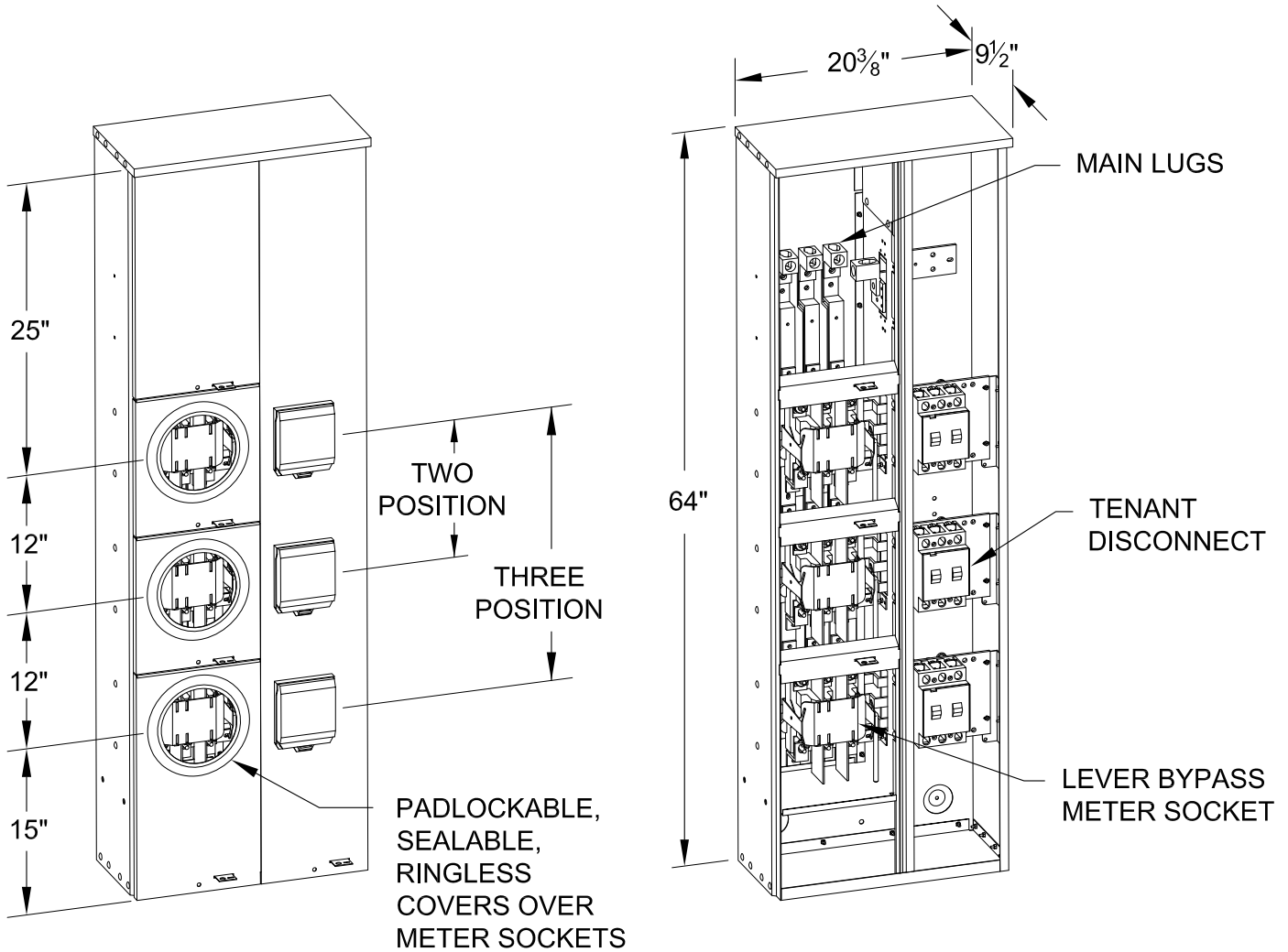
208Y/120V OR 120/240V DELTA 3Ø 4W
